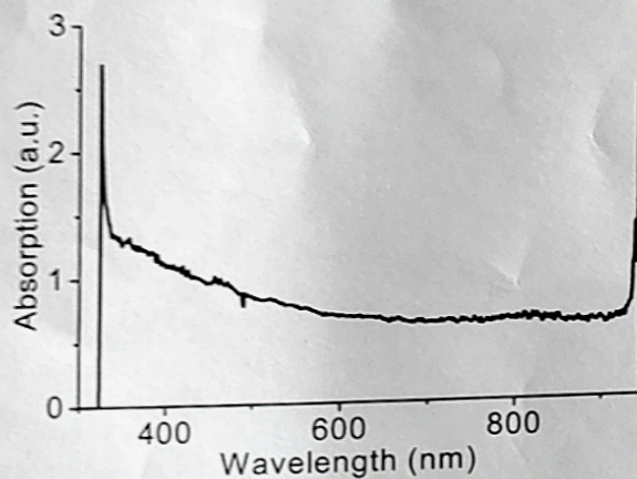
Fig. 2: Shows variation in wavelength verses % Absorption for CdO (II) thin film annealed at 600°C.
