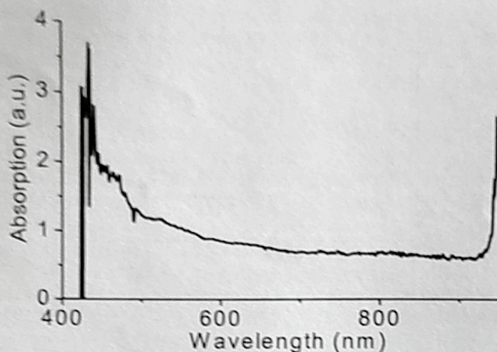
Fig. 3: Shows variation in wavelength verses % Absorption for CdO (III) thin film annealed at 750°C.
