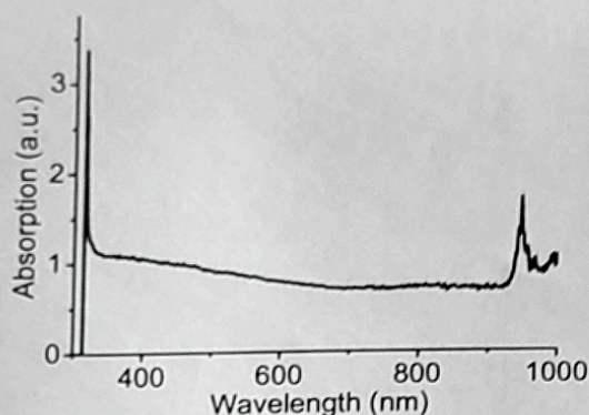
Fig. 5: Shows variation in wavelength verses % Absorption for ZnO (II) thin film annealed at 600°C.
